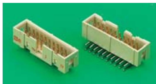
Straight Pins H=8.9mm, D=9.2mm 90° Pins H=9.2mm, D=8.9mm
