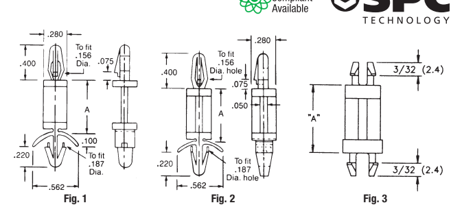
NYLON FLEXIBLE SUPPORTS – FIG. 1 Flexible supports allow access to underside of PC board for maintenance and repair. Lock to PC board and chassis. Material: nylon %. Color: natural.
