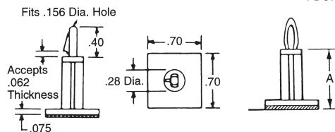
Fit 0.156" diameter hole. Accept 0.062" thickness panel. 1/32" thick double-adhesive tape with release tab. Material: nylon %. Color: natural. Sold in packages of 100.
